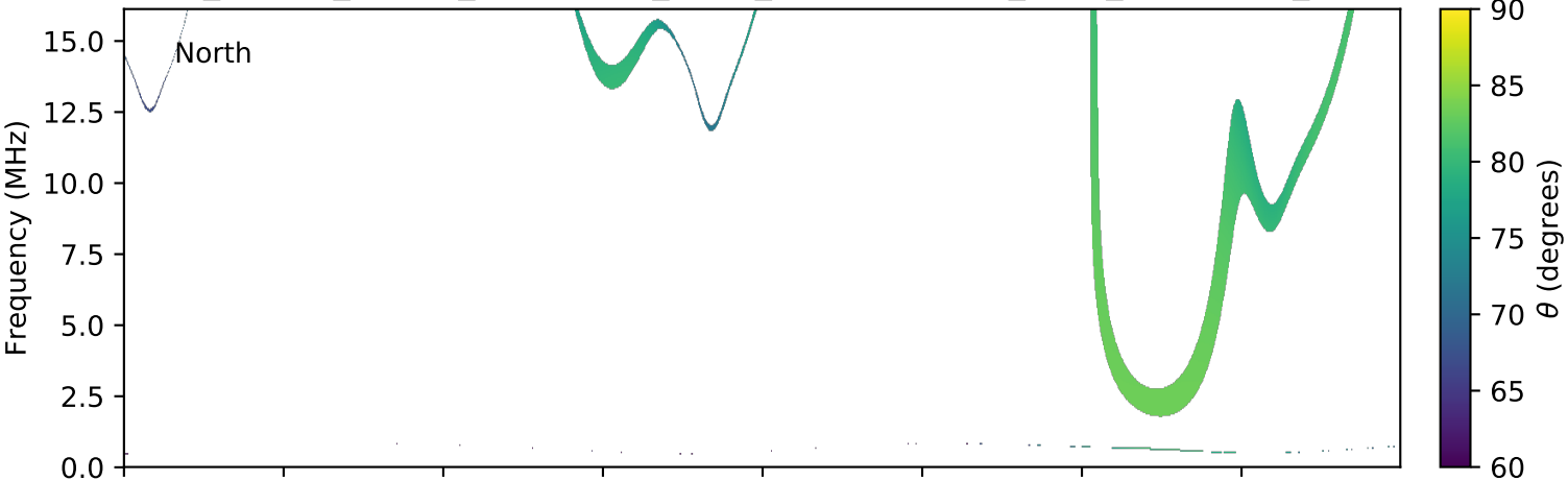
expres_cassini_jupiter_ganymede_isaac_lossc-wid1deg_3kev_20000818_v01.cdf
