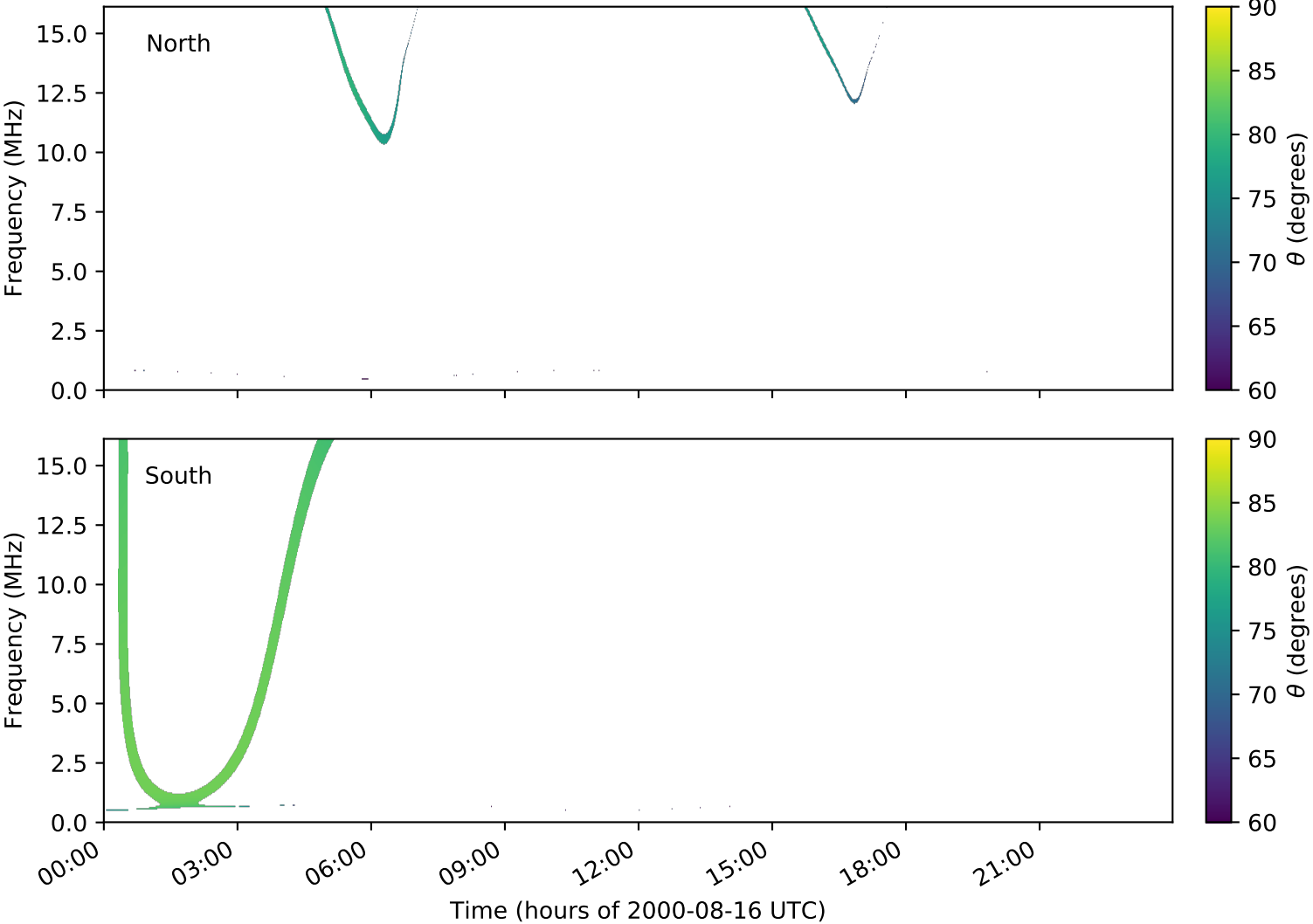
expres_cassini_jupiter_ganymede_isaac_lossc-wid1deg_3kev_20000816_v01.cdf
