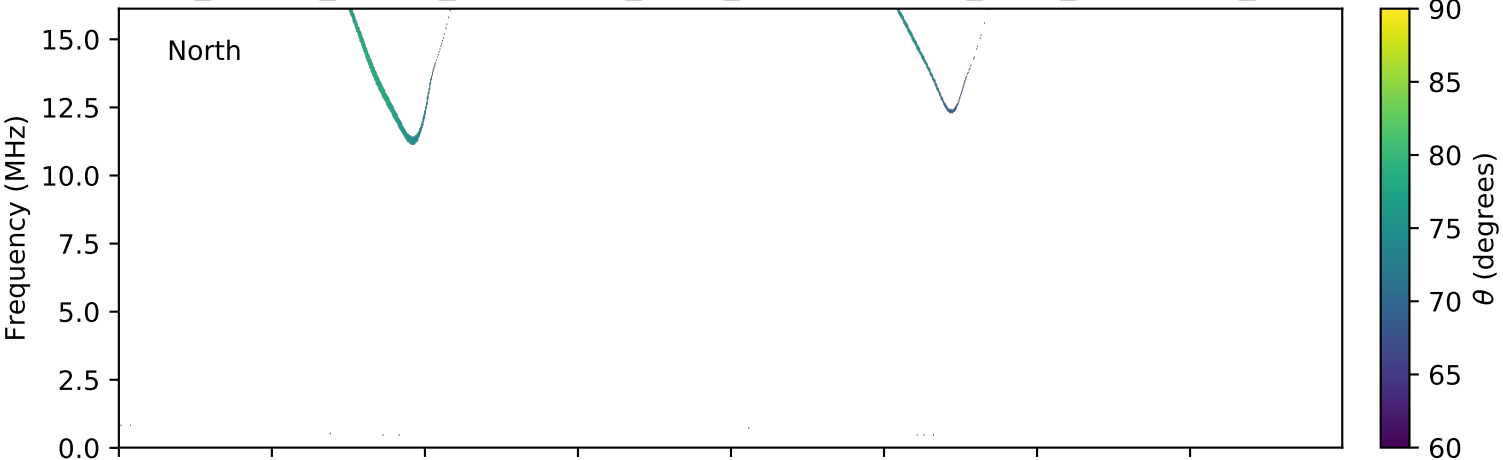
expres_cassini_jupiter_ganymede_isaac_lossc-wid1deg_3kev_20000809_v01.cdf
