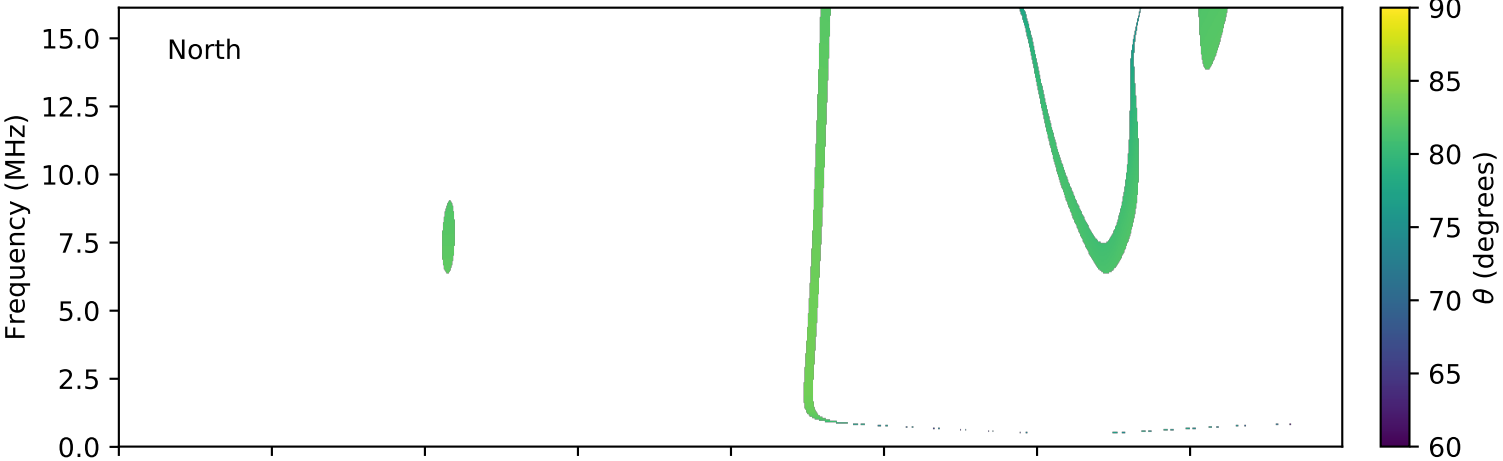
expres_cassini_jupiter_ganymede_isaac_lossc-wid1deg_3kev_20000808_v01.cdf
