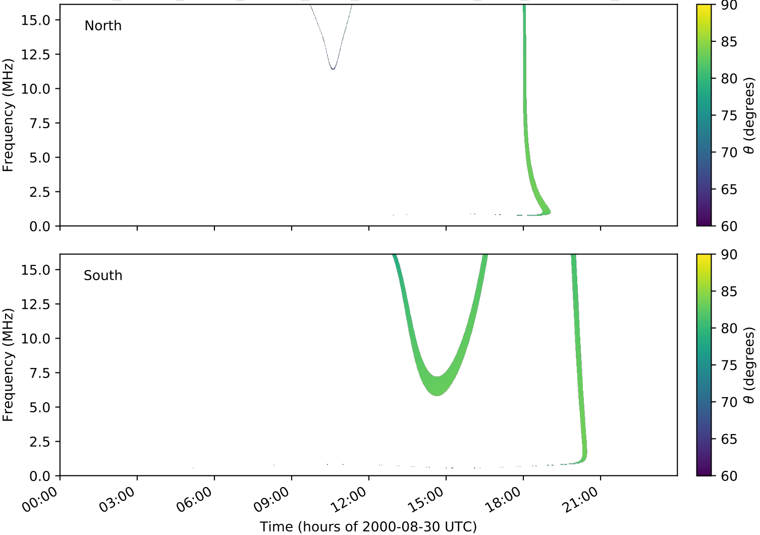
expres_cassini_jupiter_europa_isaac_lossc-wid1deg_3kev_20000830_v01.cdf
