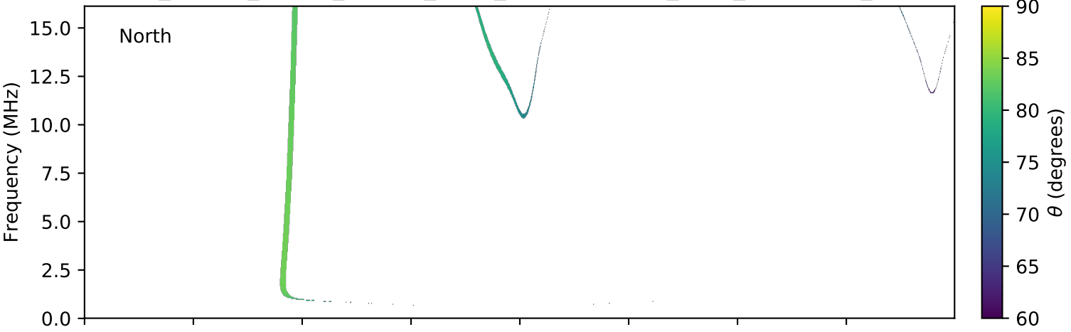
expres_cassini_jupiter_europa_isaac_lossc-wid1deg_3kev_20000829_v01.cdf
