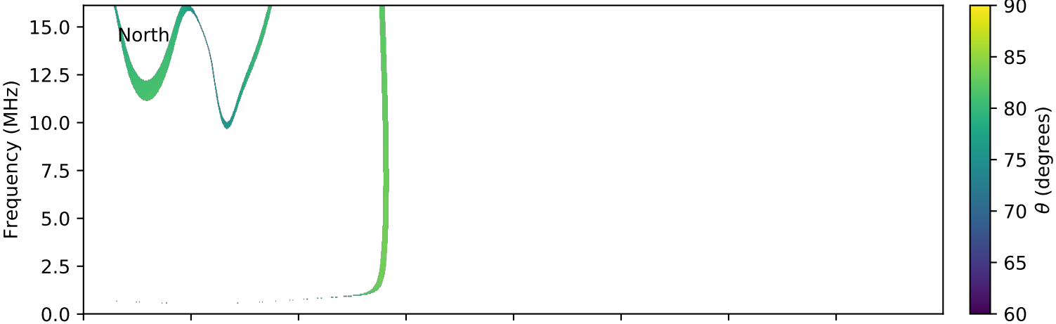
expres_cassini_jupiter_europa_isaac_lossc-wid1deg_3kev_20000827_v01.cdf
