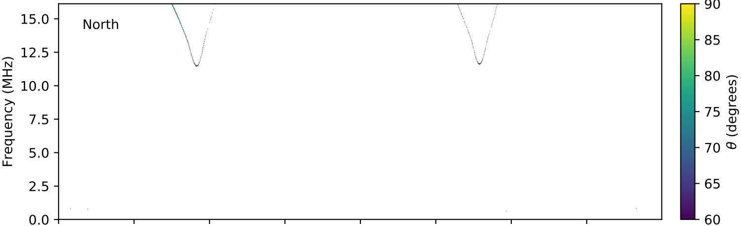
expres_cassini_jupiter_europa_isaac_lossc-wid1deg_3kev_20000826_v01.cdf
