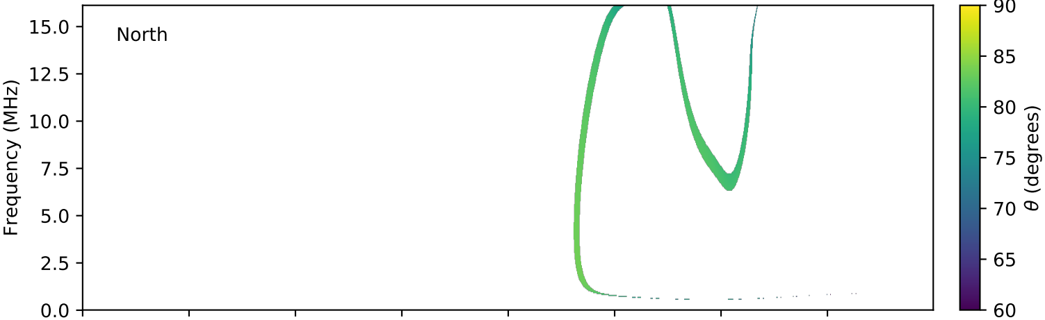
expres_cassini_jupiter_europa_isaac_lossc-wid1deg_3kev_20000825_v01.cdf
