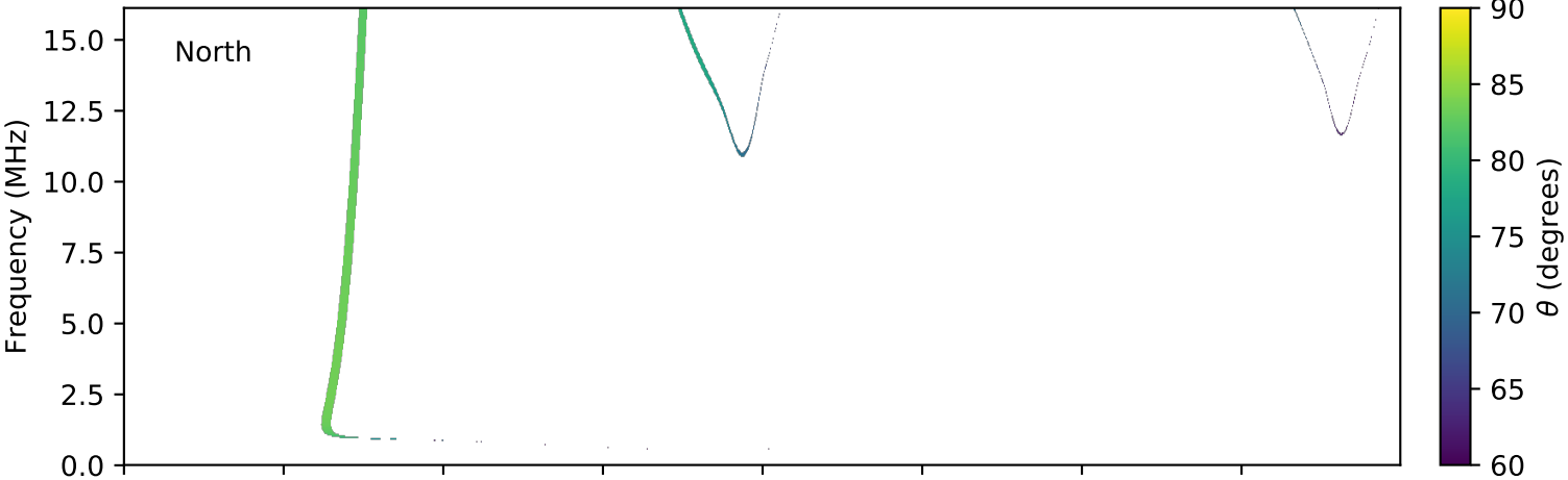
expres_cassini_jupiter_europa_isaac_lossc-wid1deg_3kev_20000822_v01.cdf
