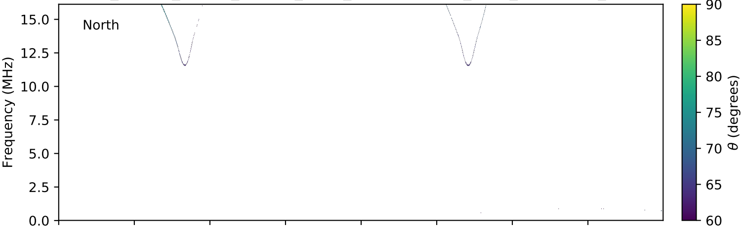
expres_cassini_jupiter_europa_isaac_lossc-wid1deg_3kev_20000819_v01.cdf
