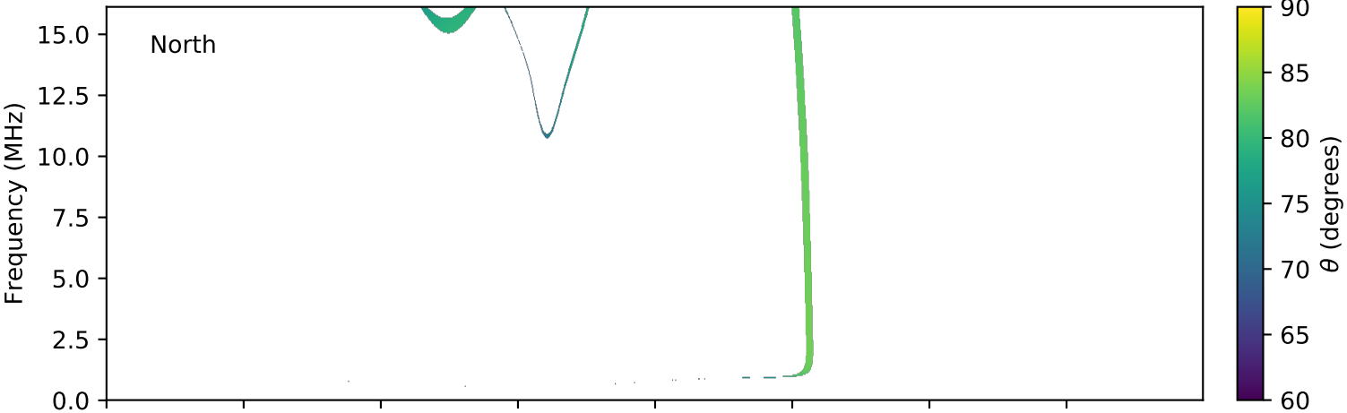
expres_cassini_jupiter_europa_isaac_lossc-wid1deg_3kev_20000816_v01.cdf
