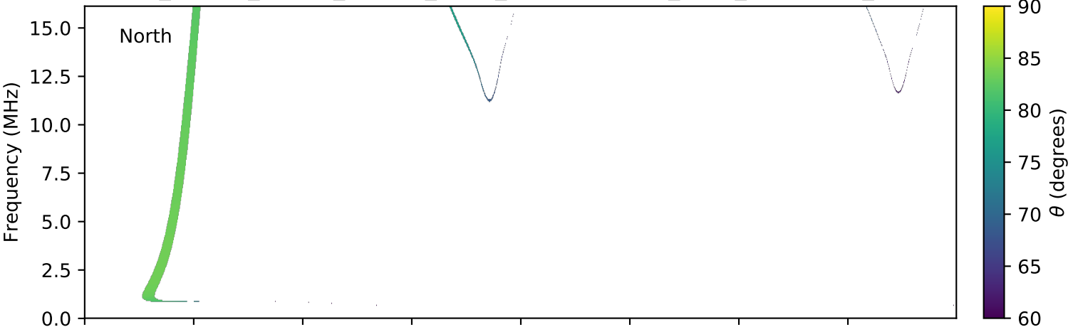
expres_cassini_jupiter_europa_isaac_lossc-wid1deg_3kev_20000815_v01.cdf
