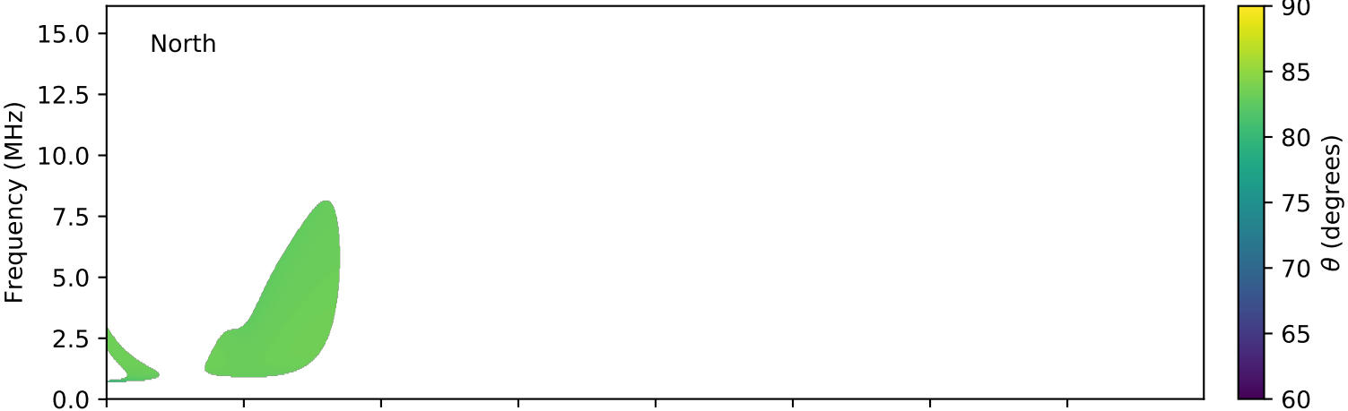
expres_cassini_jupiter_europa_isaac_lossc-wid1deg_3kev_20000813_v01.cdf
