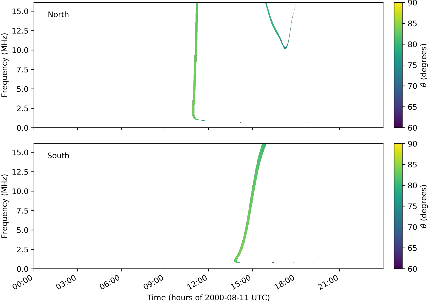
expres_cassini_jupiter_europa_isaac_lossc-wid1deg_3kev_20000811_v01.cdf
