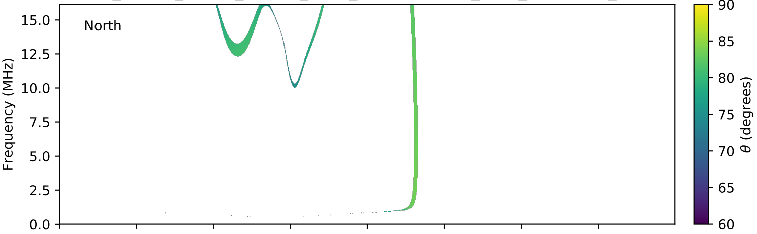
expres_cassini_jupiter_europa_isaac_lossc-wid1deg_3kev_20000809_v01.cdf
