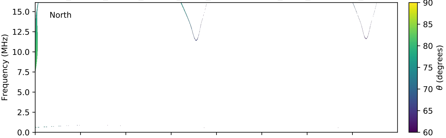
expres_cassini_jupiter_europa_isaac_lossc-wid1deg_3kev_20000808_v01.cdf
