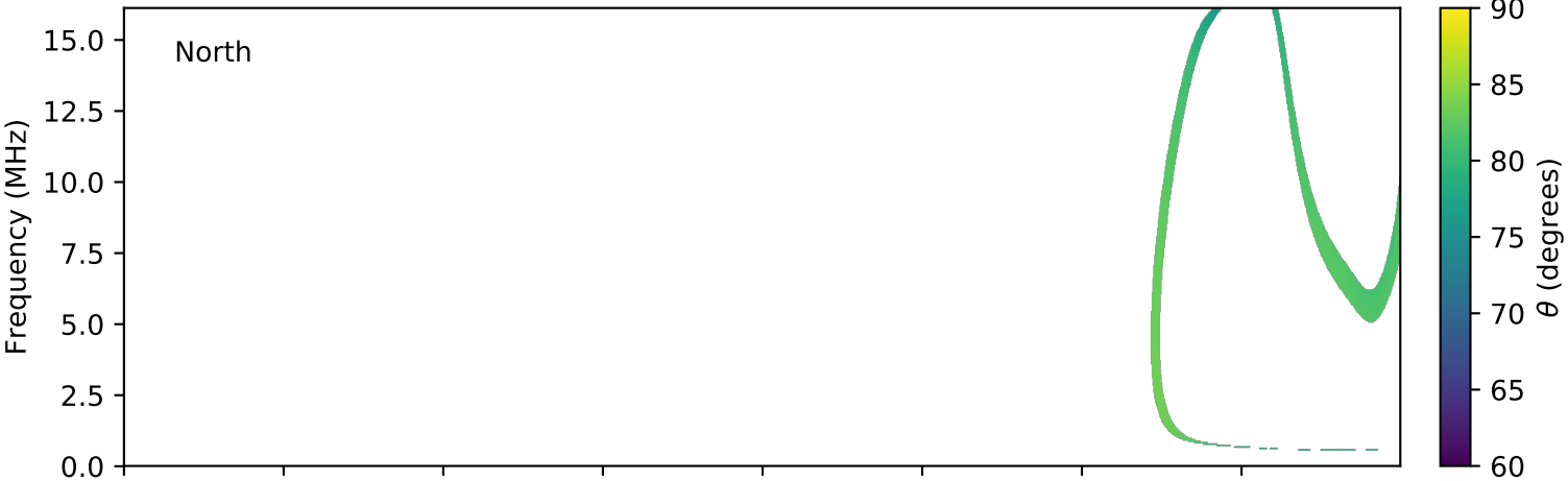
expres_cassini_jupiter_europa_isaac_lossc-wid1deg_3kev_20000807_v01.cdf
