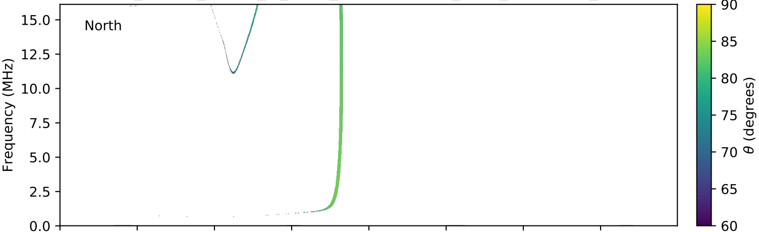
expres_cassini_jupiter_io_isaac_lossc-wid1deg_3kev_20000731_v01.cdf
