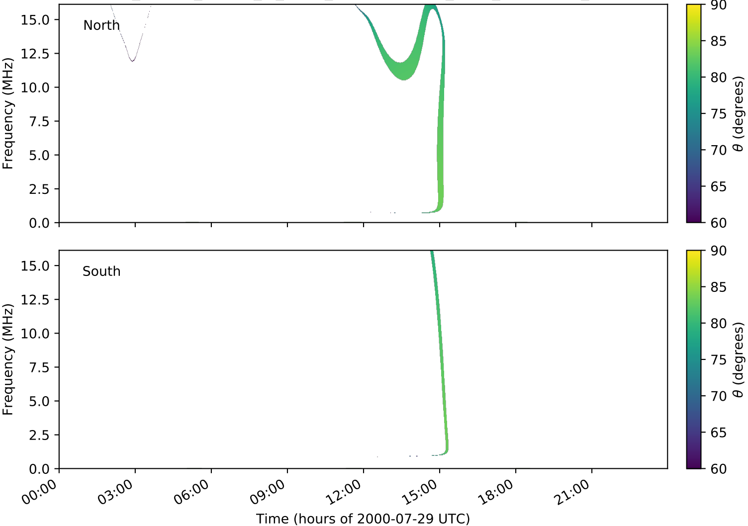
expres_cassini_jupiter_io_isaac_lossc-wid1deg_3kev_20000729_v01.cdf
