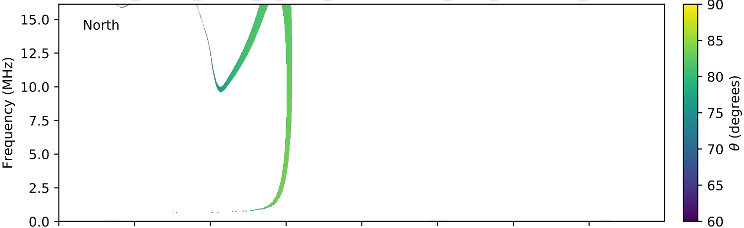
expres_cassini_jupiter_io_isaac_lossc-wid1deg_3kev_20000724_v01.cdf
