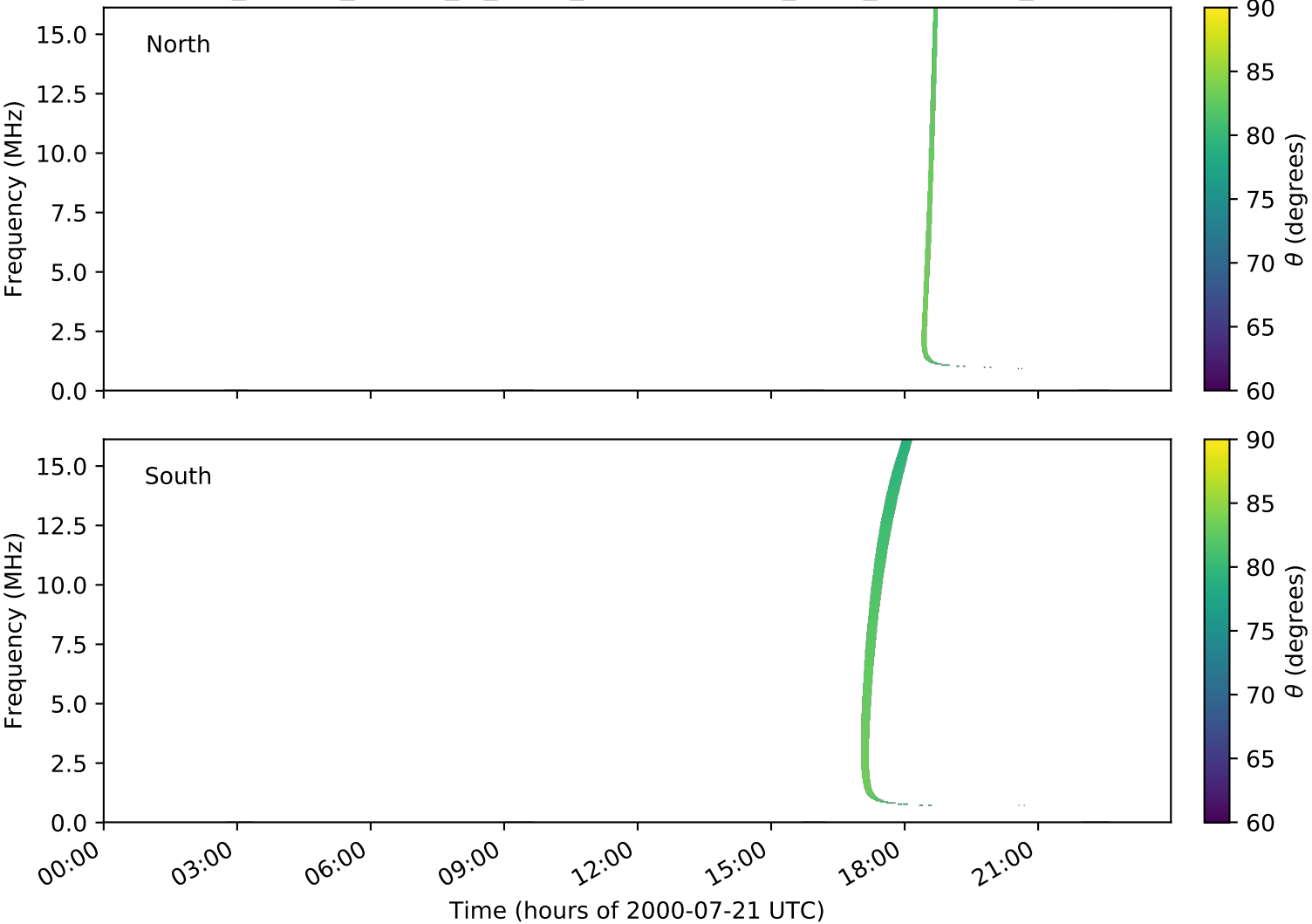
expres_cassini_jupiter_io_isaac_lossc-wid1deg_3kev_20000721_v01.cdf
