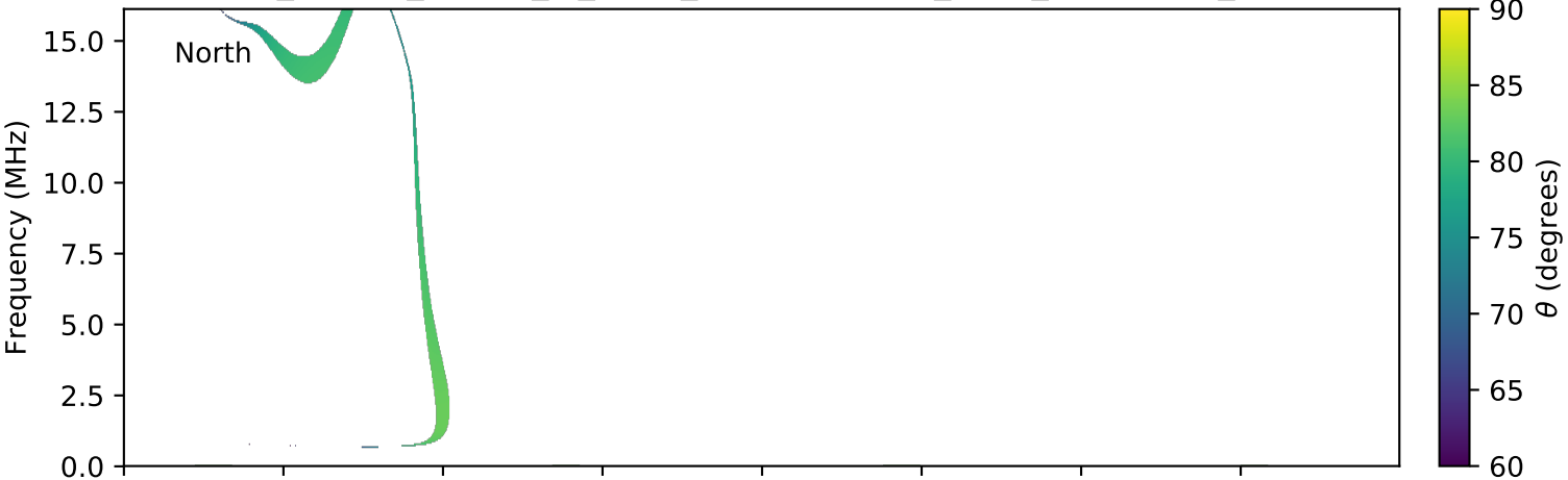
expres_cassini_jupiter_io_isaac_lossc-wid1deg_3kev_20000717_v01.cdf
