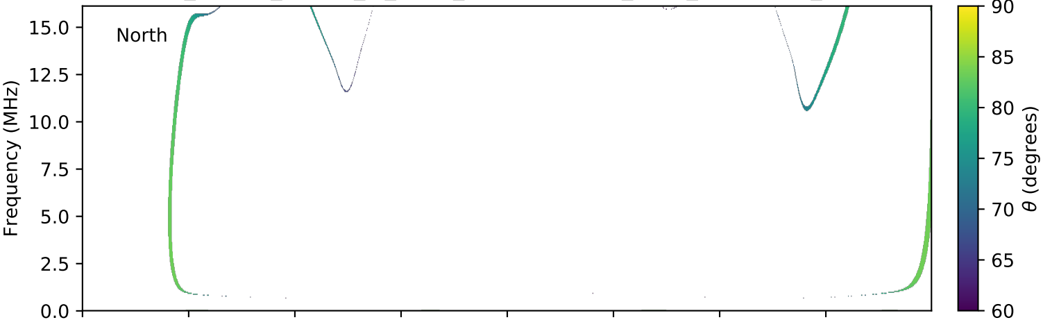
expres_cassini_jupiter_io_isaac_lossc-wid1deg_3kev_20000711_v01.cdf
