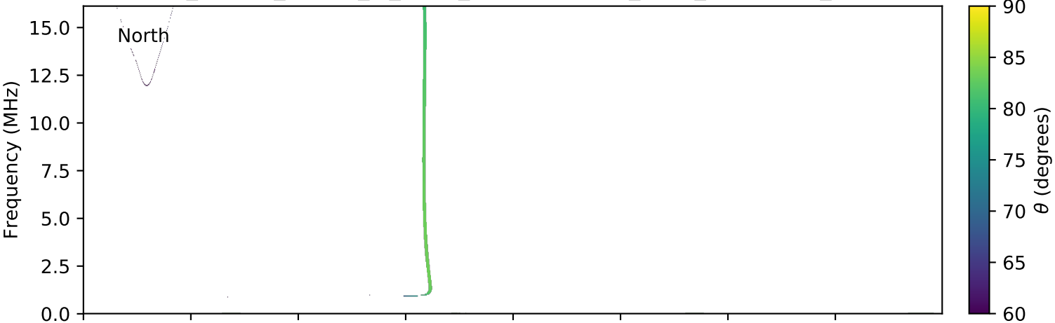
expres_cassini_jupiter_io_isaac_lossc-wid1deg_3kev_20000708_v01.cdf
