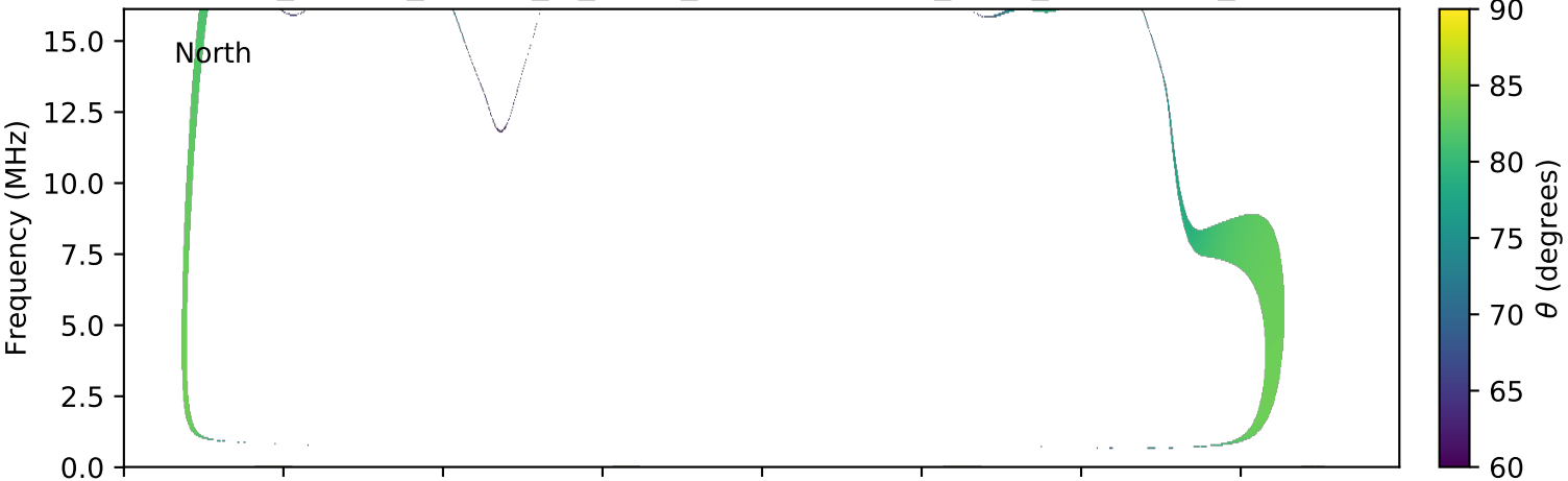
expres_cassini_jupiter_io_isaac_lossc-wid1deg_3kev_20000704_v01.cdf
