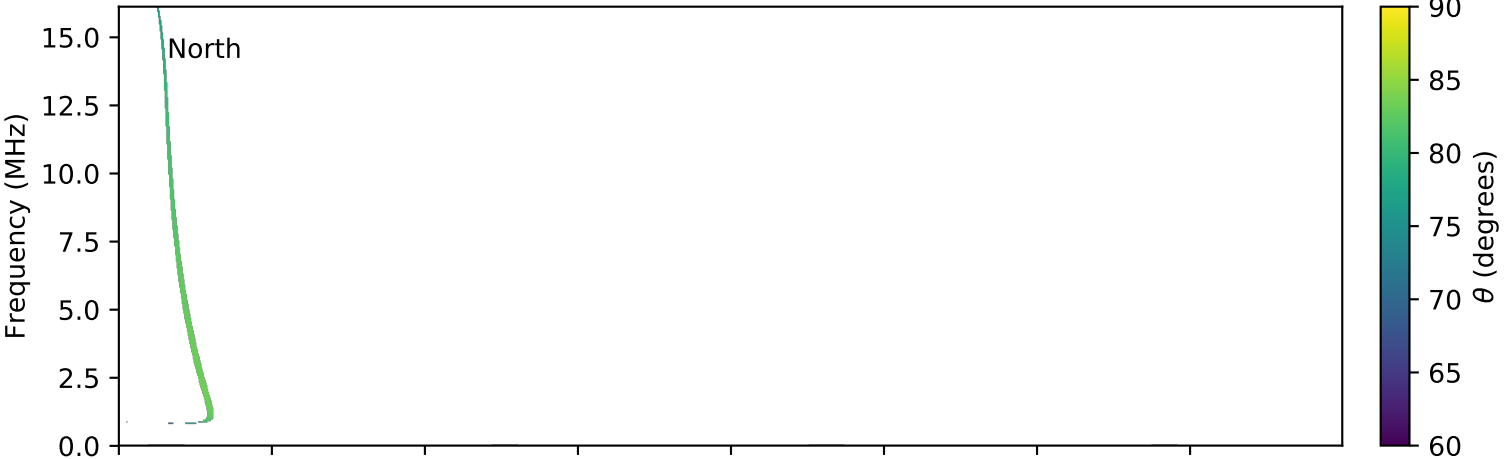
expres_cassini_jupiter_io_isaac_lossc-wid1deg_3kev_20000703_v01.cdf
