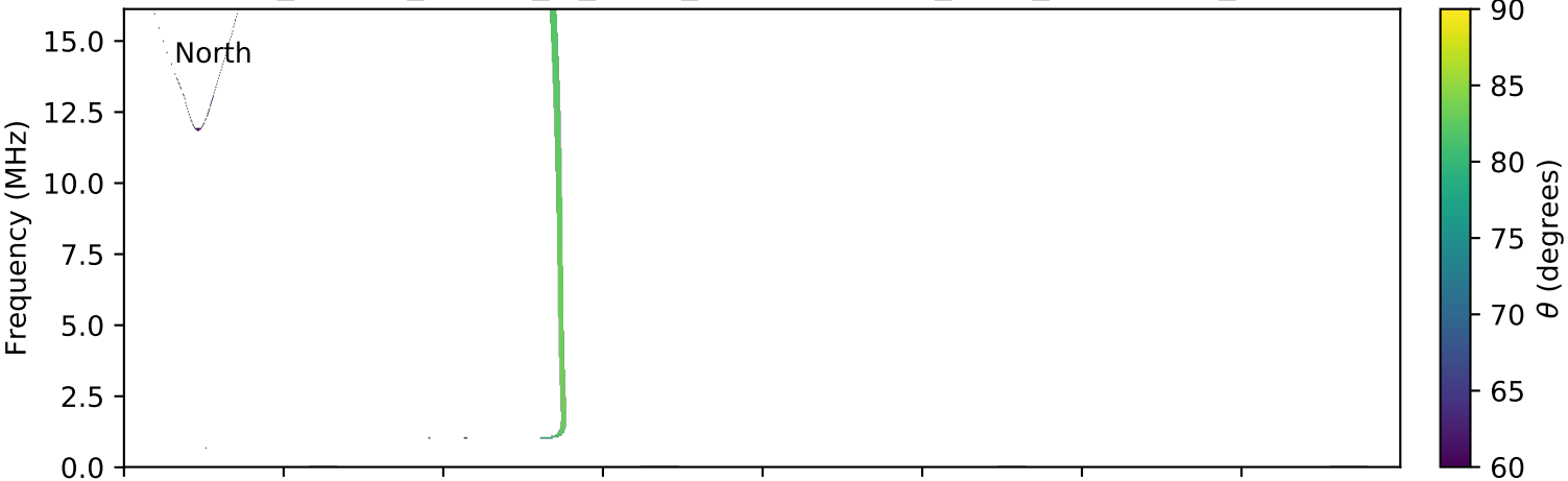
expres_cassini_jupiter_io_isaac_lossc-wid1deg_3kev_20000701_v01.cdf
