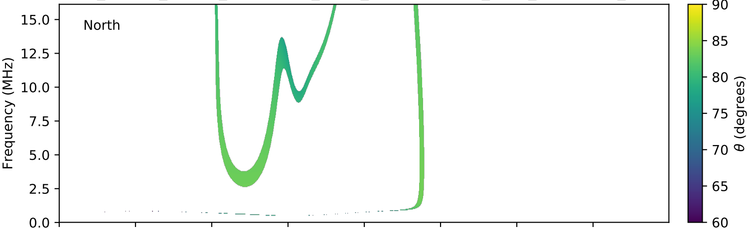
expres_cassini_jupiter_ganymede_isaac_lossc-wid1deg_3kev_20000728_v01.cdf
