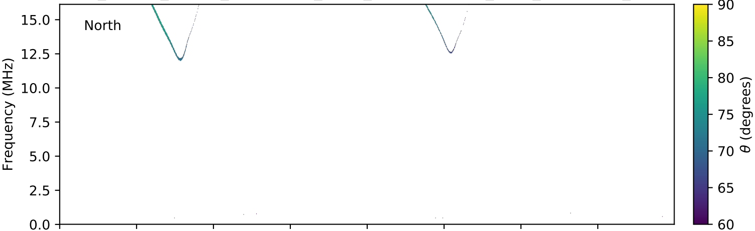
expres_cassini_jupiter_ganymede_isaac_lossc-wid1deg_3kev_20000726_v01.cdf
