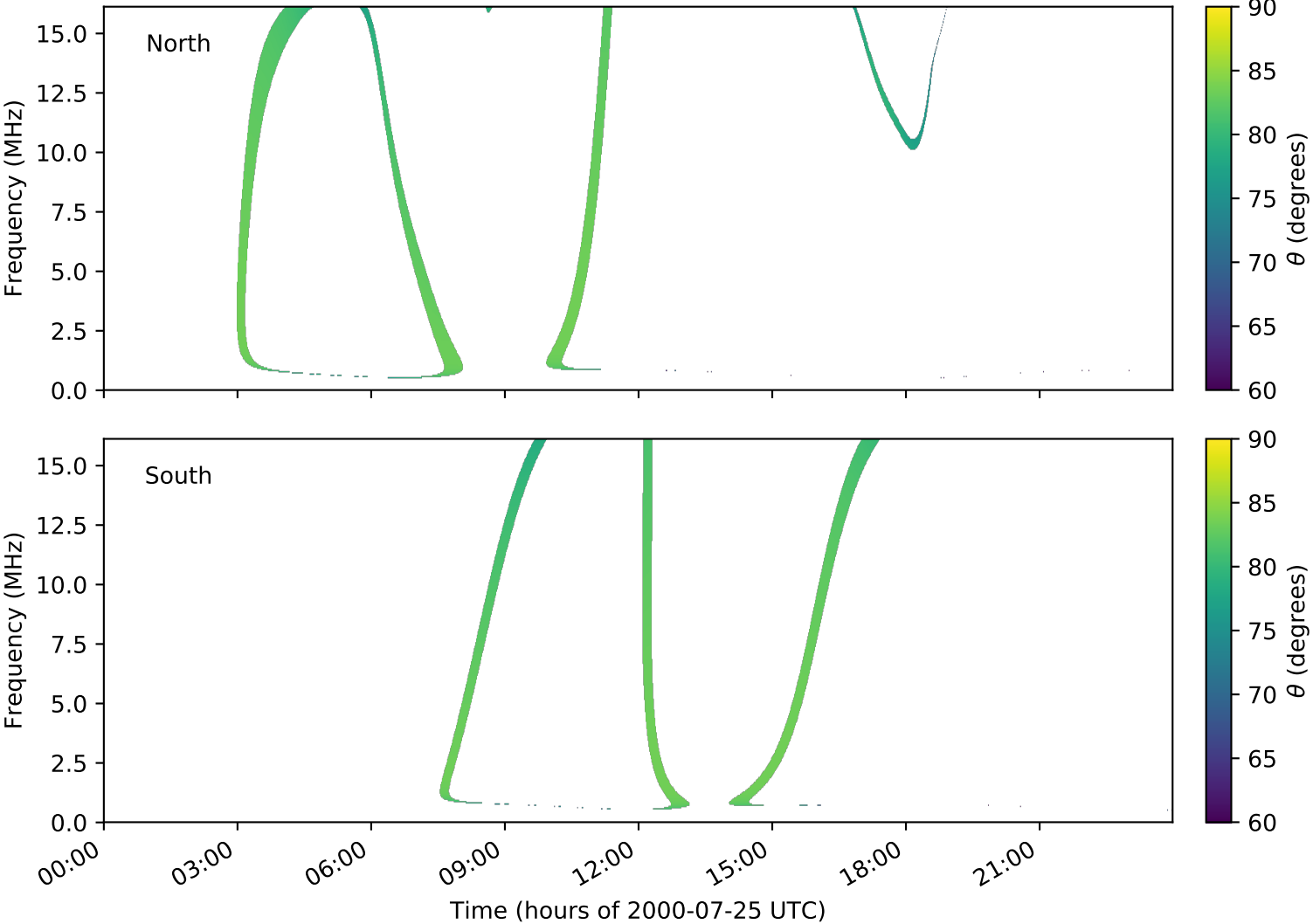
expres_cassini_jupiter_ganymede_isaac_lossc-wid1deg_3kev_20000725_v01.cdf
