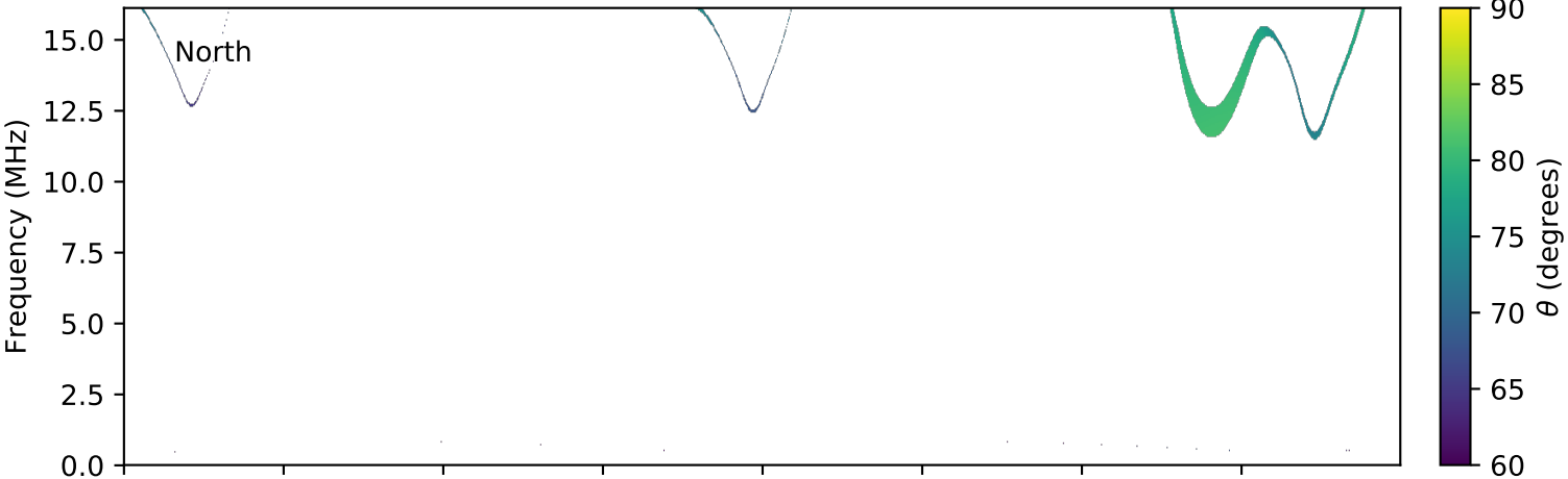
expres_cassini_jupiter_ganymede_isaac_lossc-wid1deg_3kev_20000720_v01.cdf
