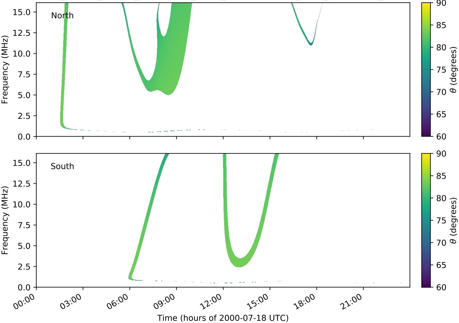
expres_cassini_jupiter_ganymede_isaac_lossc-wid1deg_3kev_20000718_v01.cdf
