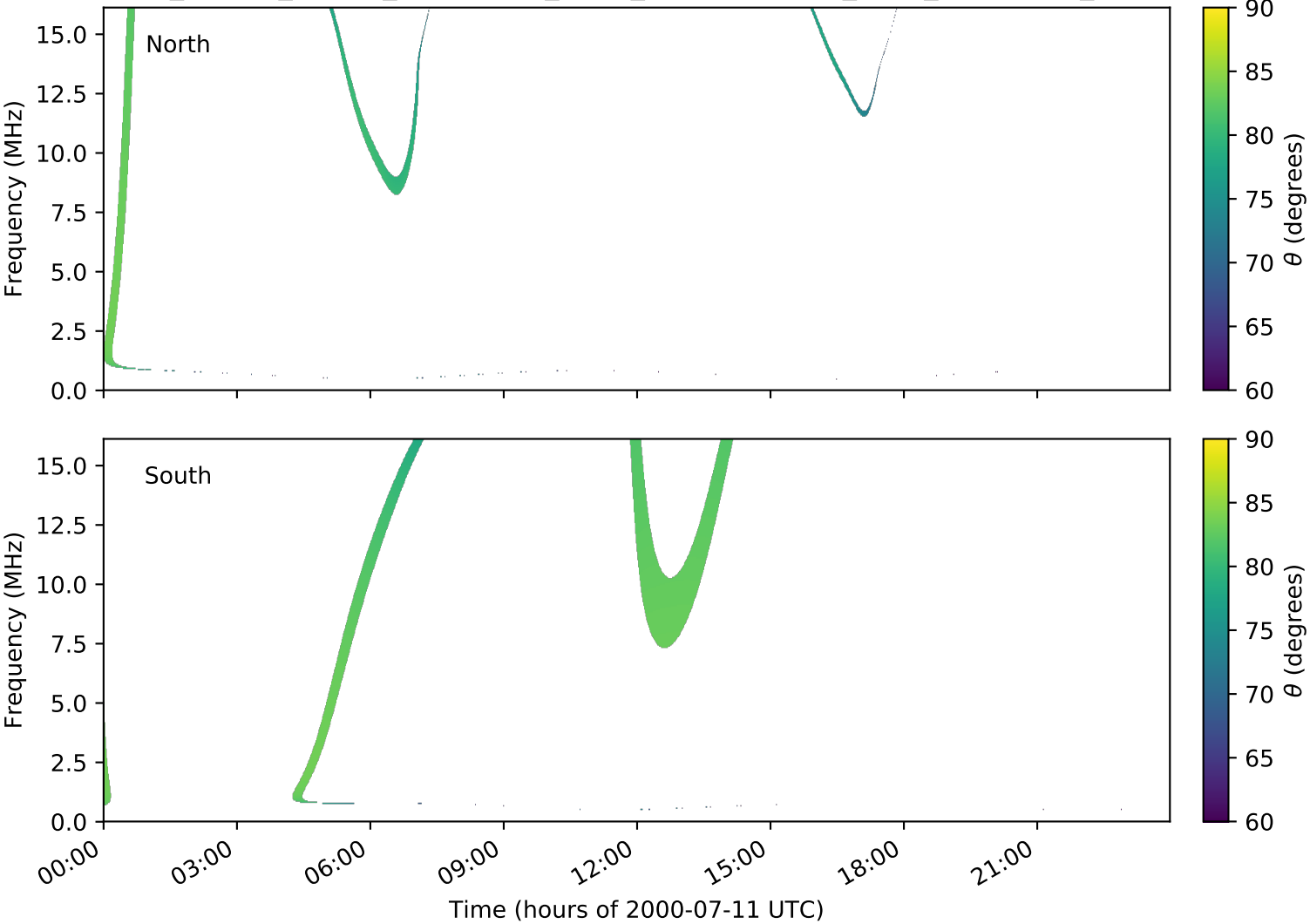
expres_cassini_jupiter_ganymede_isaac_lossc-wid1deg_3kev_20000711_v01.cdf
