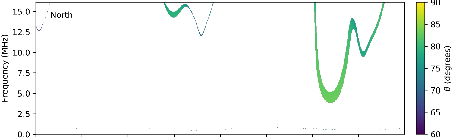
expres_cassini_jupiter_ganymede_isaac_lossc-wid1deg_3kev_20000706_v01.cdf
