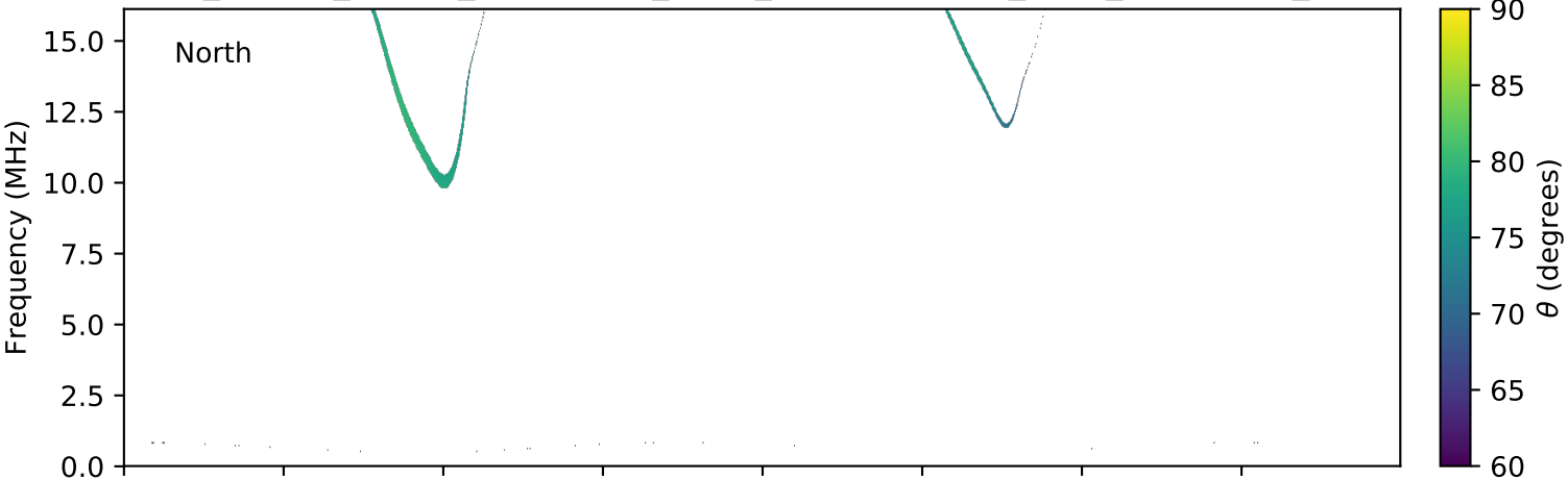
expres_cassini_jupiter_ganymede_isaac_lossc-wid1deg_3kev_20000704_v01.cdf
