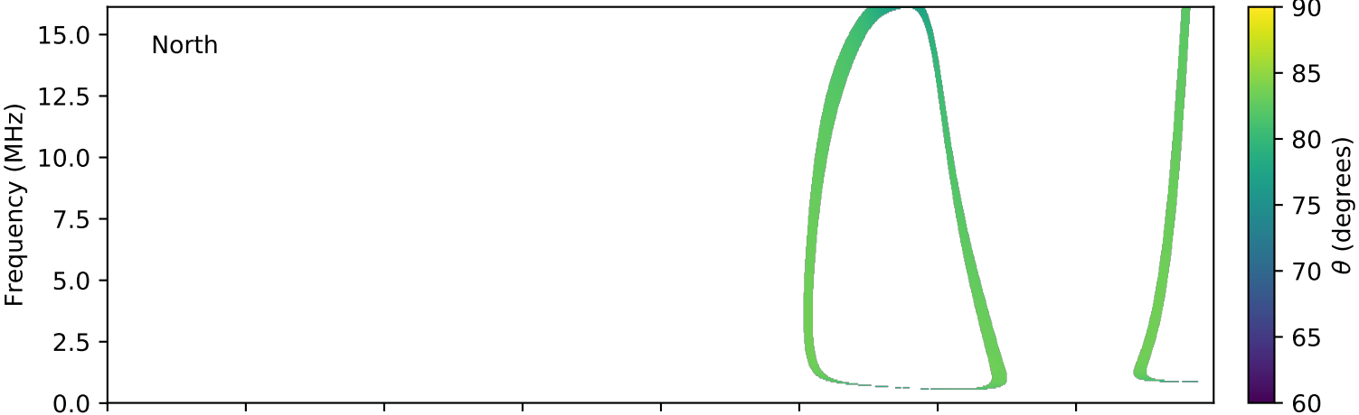
expres_cassini_jupiter_ganymede_isaac_lossc-wid1deg_3kev_20000703_v01.cdf
