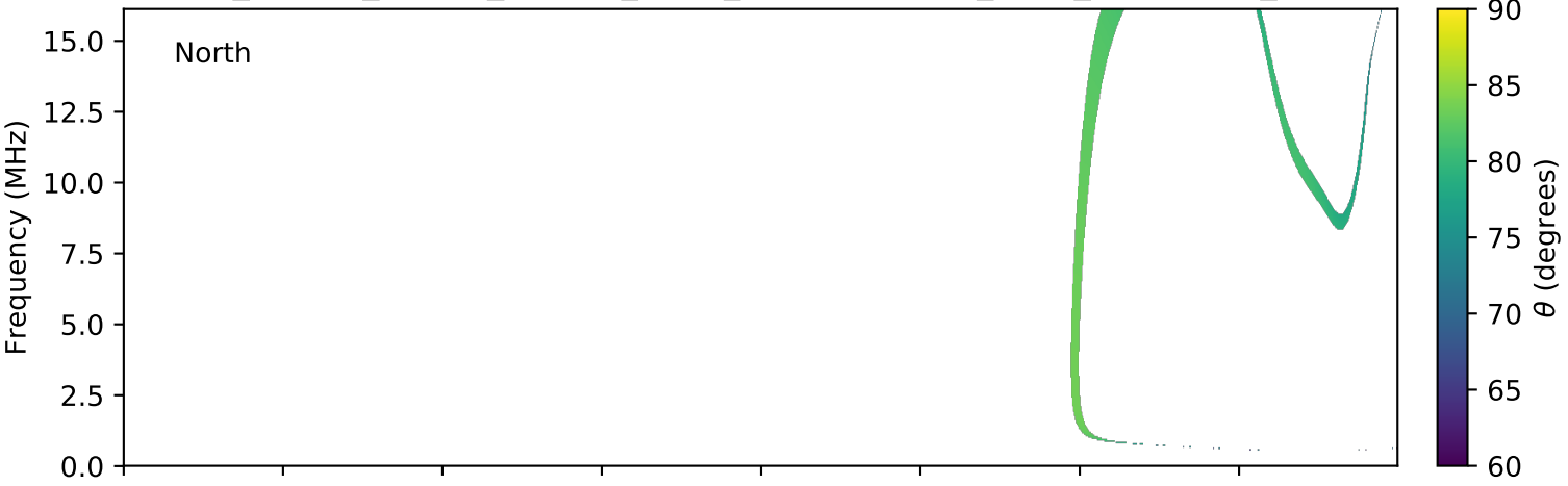
expres_cassini_jupiter_europa_isaac_lossc-wid1deg_3kev_20000731_v01.cdf
