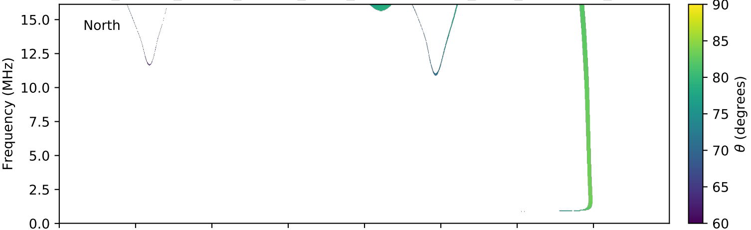
expres_cassini_jupiter_europa_isaac_lossc-wid1deg_3kev_20000729_v01.cdf
