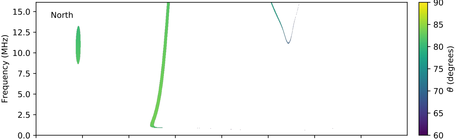
expres_cassini_jupiter_europa_isaac_lossc-wid1deg_3kev_20000728_v01.cdf
