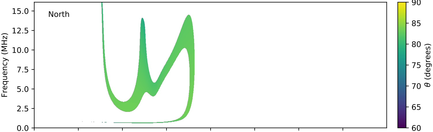
expres_cassini_jupiter_europa_isaac_lossc-wid1deg_3kev_20000726_v01.cdf
