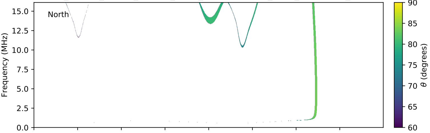
expres_cassini_jupiter_europa_isaac_lossc-wid1deg_3kev_20000722_v01.cdf
