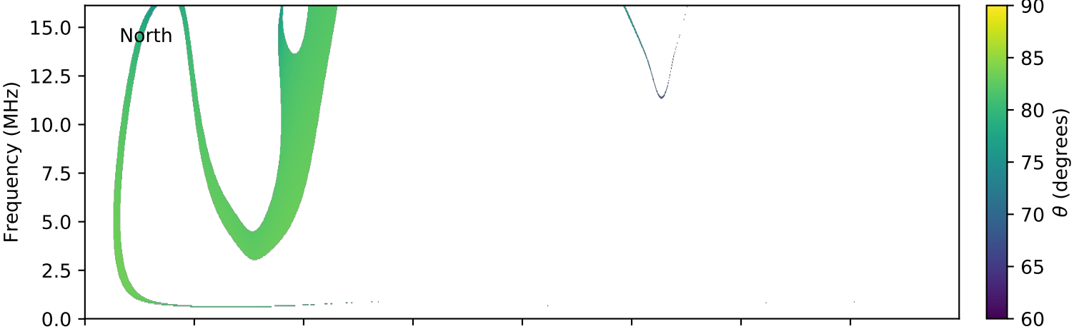
expres_cassini_jupiter_europa_isaac_lossc-wid1deg_3kev_20000721_v01.cdf
