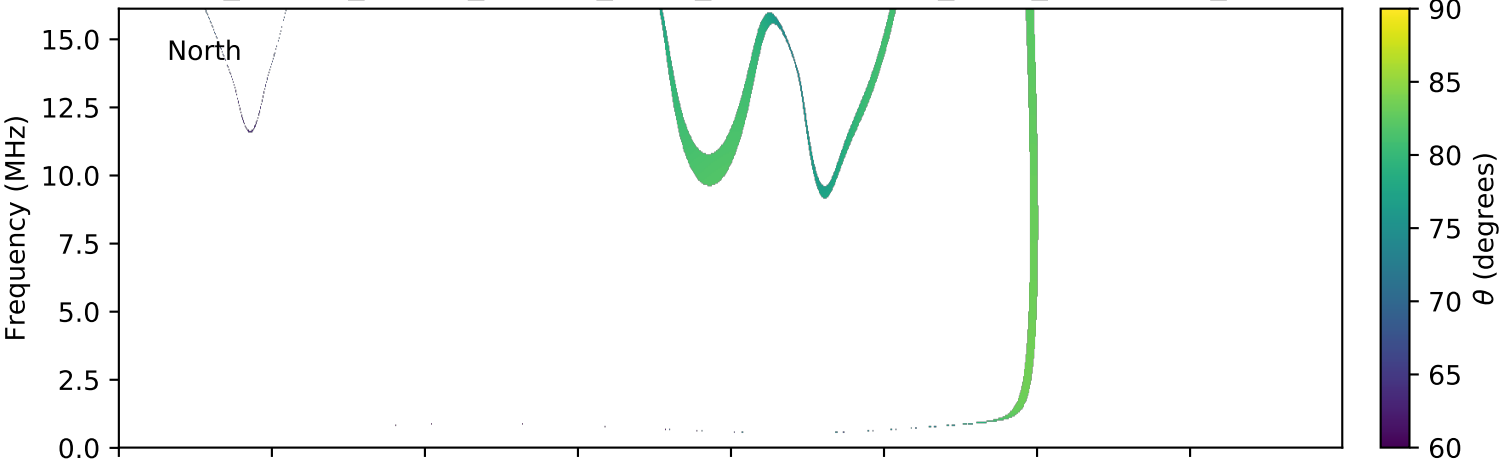
expres_cassini_jupiter_europa_isaac_lossc-wid1deg_3kev_20000715_v01.cdf
