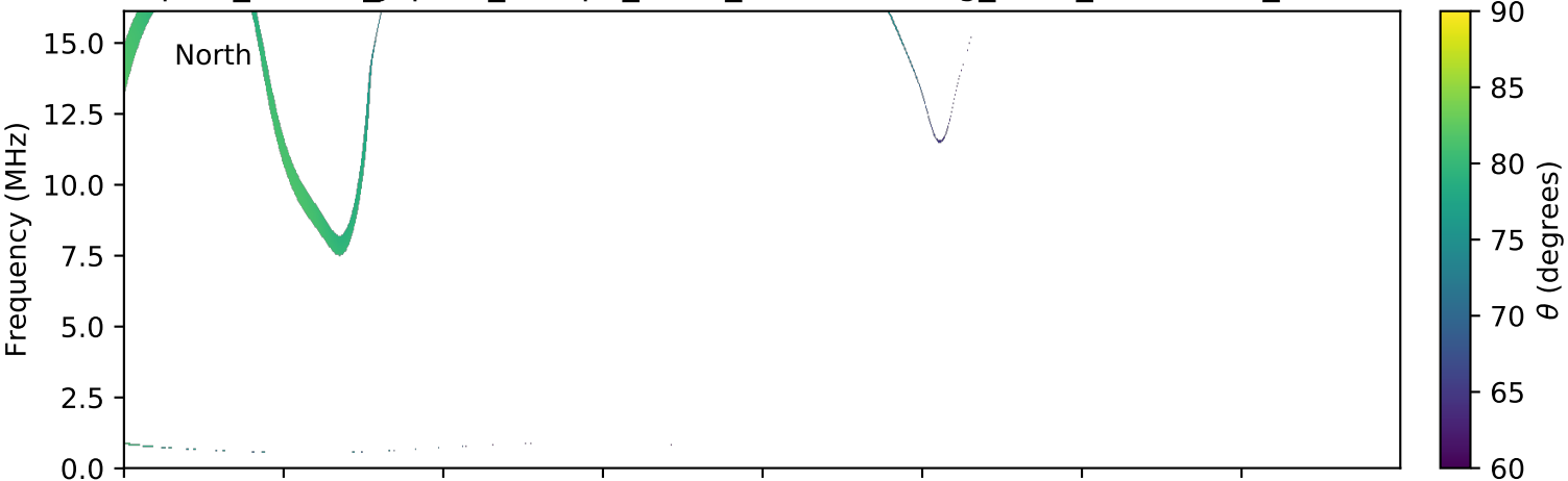
expres_cassini_jupiter_europa_isaac_lossc-wid1deg_3kev_20000714_v01.cdf
