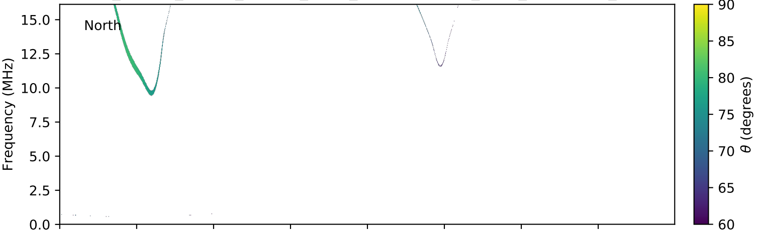
expres_cassini_jupiter_europa_isaac_lossc-wid1deg_3kev_20000707_v01.cdf
