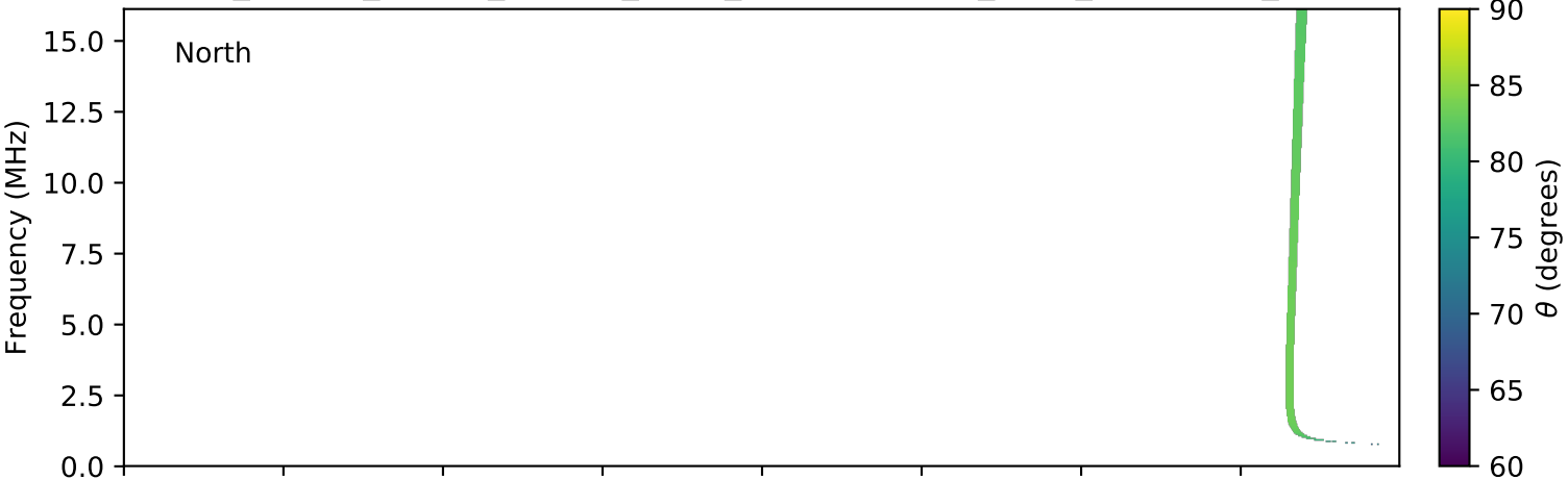
expres_cassini_jupiter_europa_isaac_lossc-wid1deg_3kev_20000706_v01.cdf
