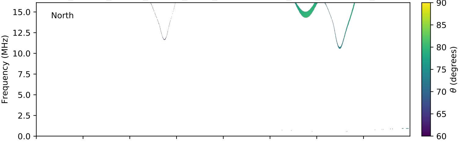
expres_cassini_jupiter_europa_isaac_lossc-wid1deg_3kev_20000704_v01.cdf
