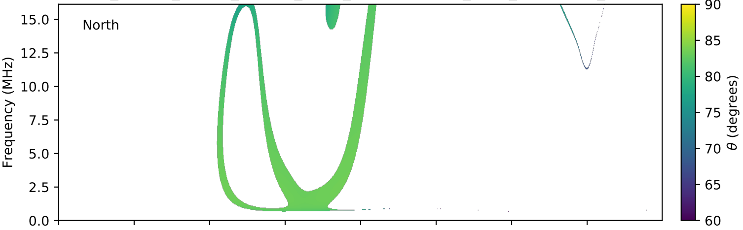
expres_cassini_jupiter_europa_isaac_lossc-wid1deg_3kev_20000703_v01.cdf
