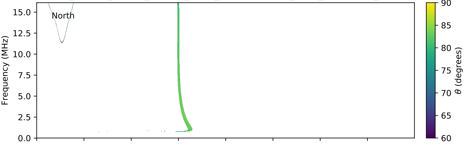
expres_cassini_jupiter_europa_isaac_lossc-wid1deg_3kev_20000701_v01.cdf
